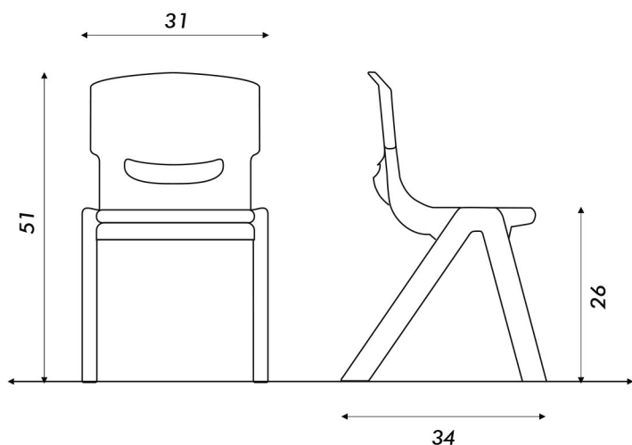
VISTA FRONTAL
